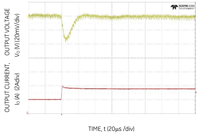
Figure 16. Transient Response to Dynamic Load Change from 50% to 100% at 12Vin, Cout=5x47uF, CTune=4.7nF, RTune=300
