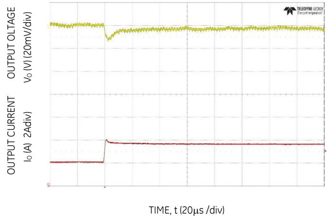
Figure 4. Transient Response to Dynamic Load Change from 50% to 100% at 12V in , C out =4x47uF+2x330uF, C Tune =15nF, R Tune =300
