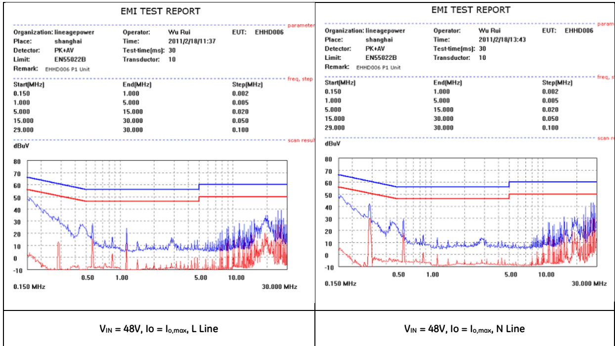
Figure 25. EMC Considerations
