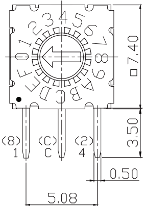
16 POSITION
