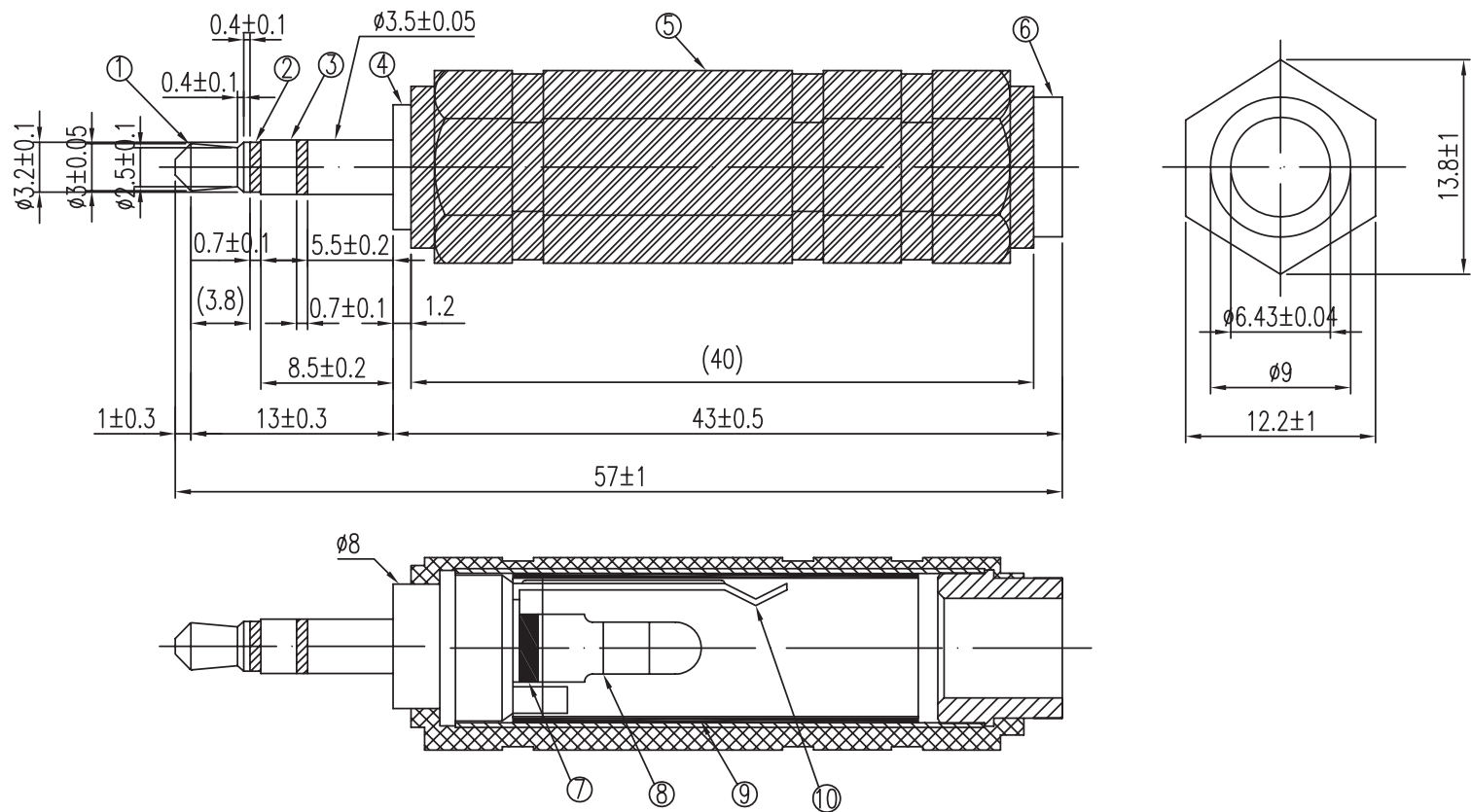
Ø3.5 Stereo Plug
