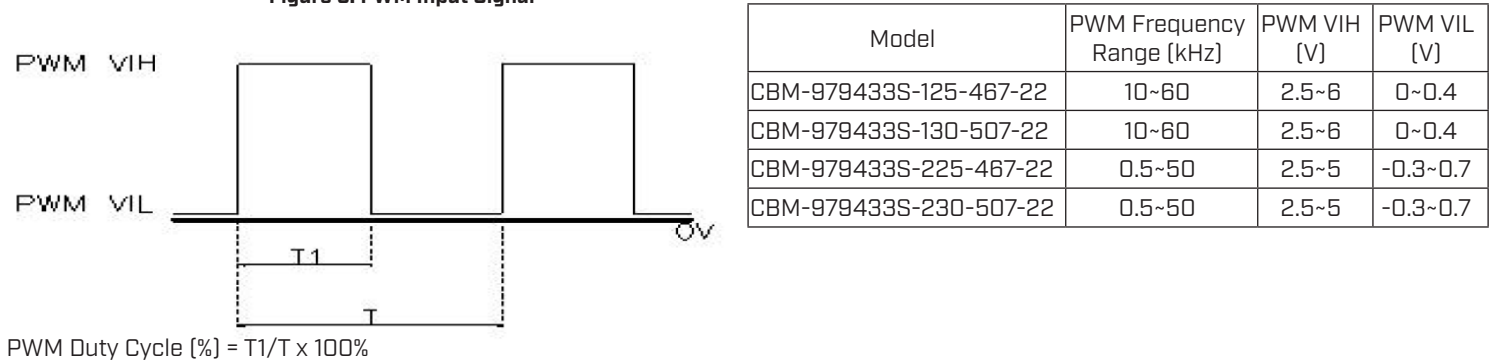
Figure 3: PWM Input Signal
