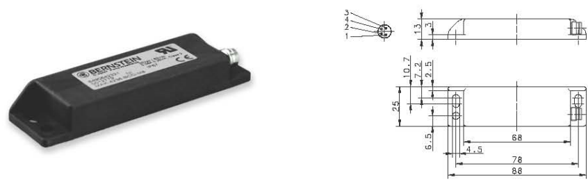
2) MAK 42 sensor, 4 pin M8 connector on the right
