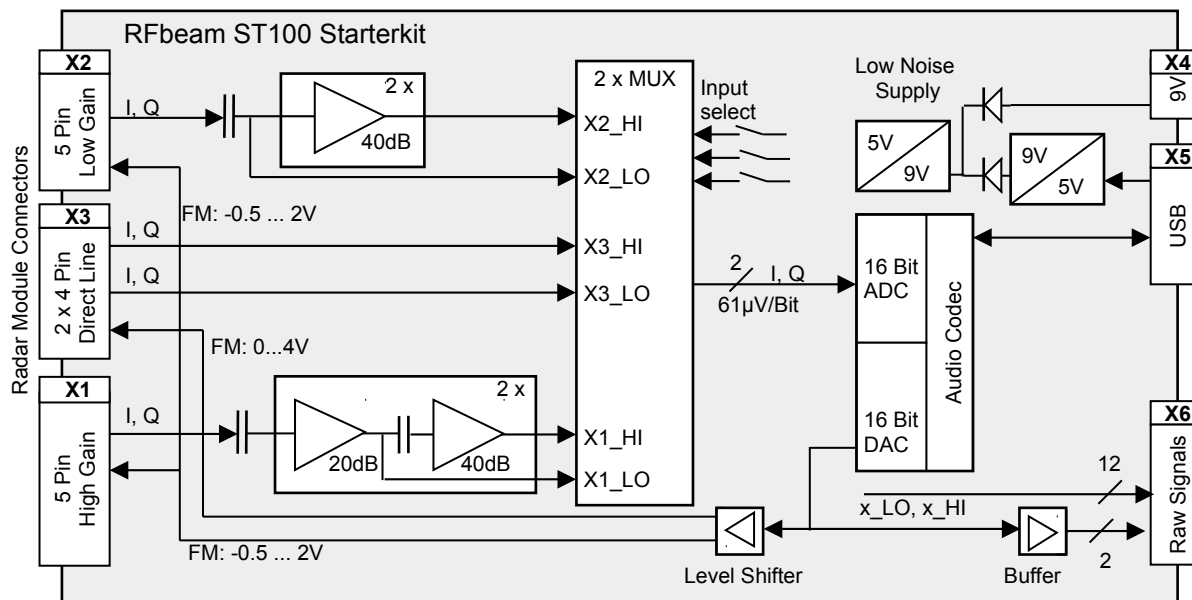
Fig. 4: Block diagram
