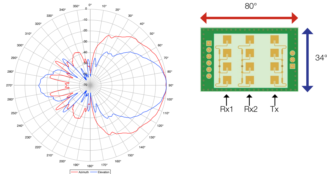
Figure 2: Antenna characteristics
