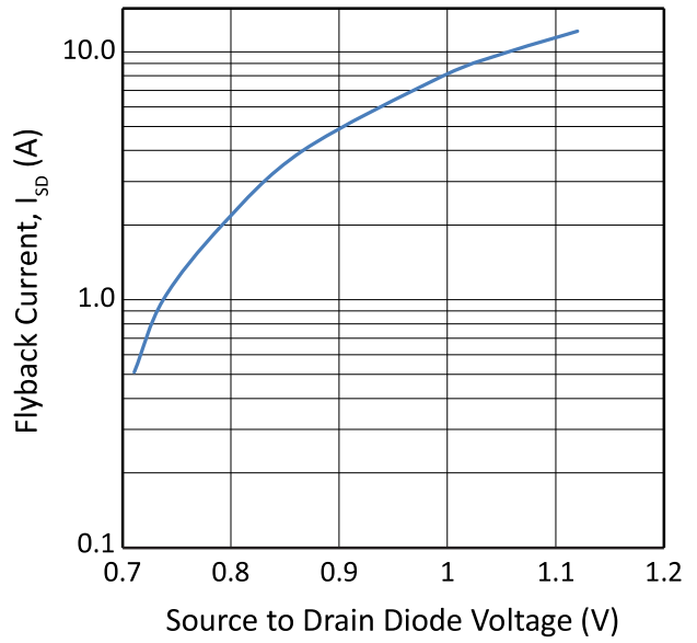
Figure 12: Reverse Diode
