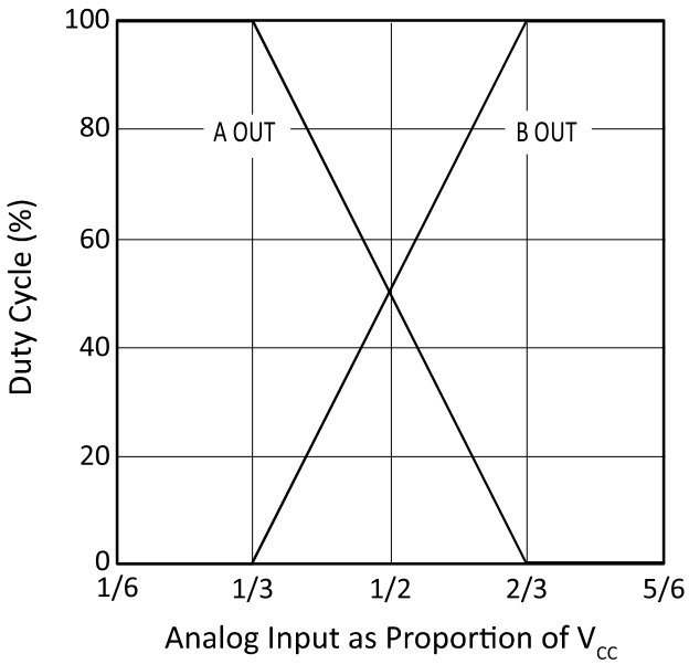
Figure 13: Duty Cycle vs. Analog Input
