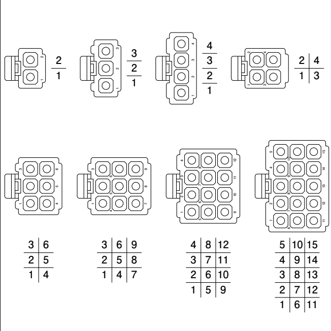
Plug housing
