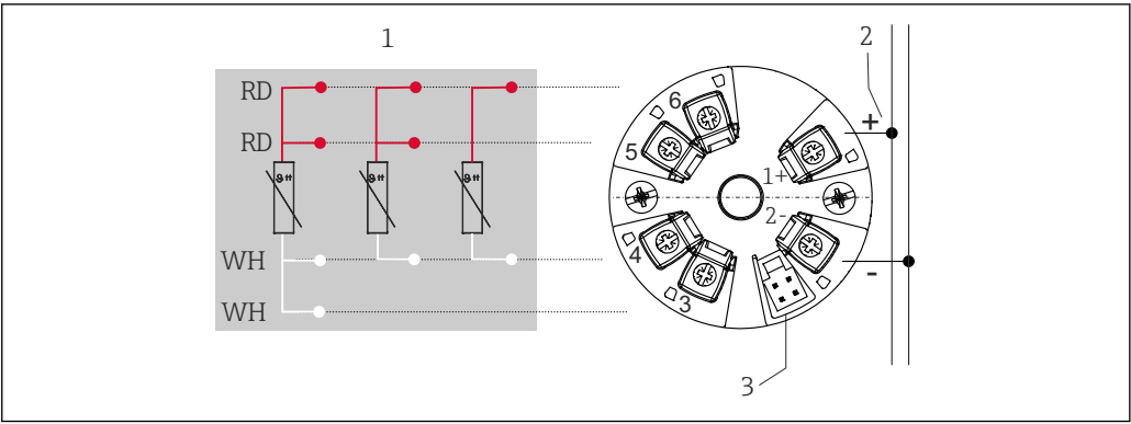
3 Terminal assignment of head transmitter
