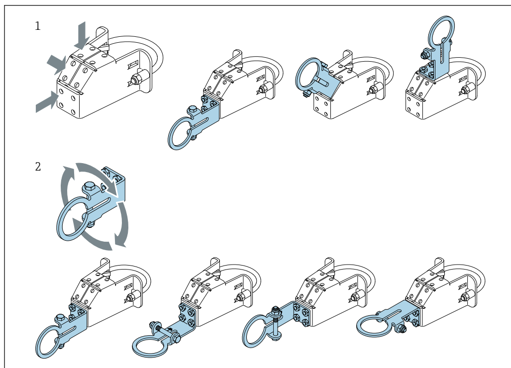
17 Alignment options via support bracket
