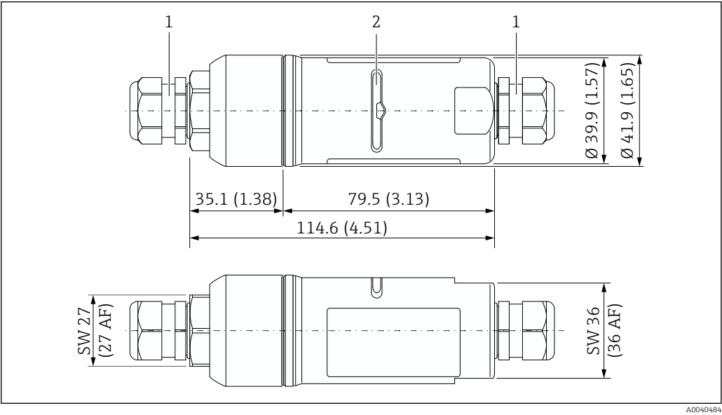
13 Dimensions of "remote mounting" version in mm (in)
