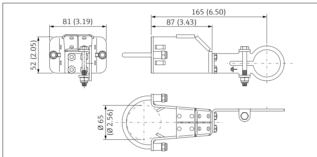
18 Dimensions of mounting bracket - pipe mounting
