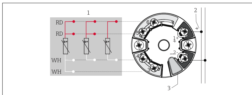
2 Head-mounted transmitter TMT7x or TMT31 (single input)
