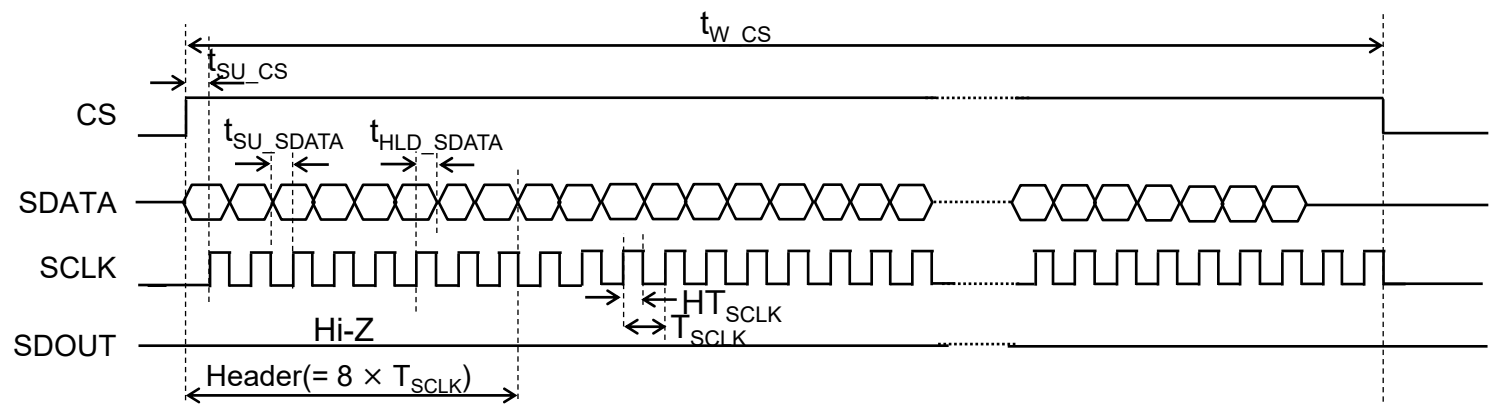
SPI Write case
