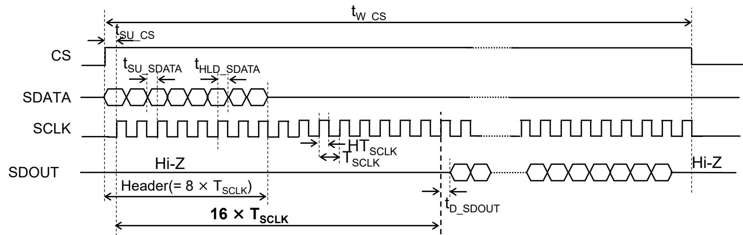
SPI Read case
