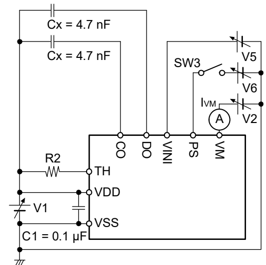
Figure 8 Test Circuit 4
