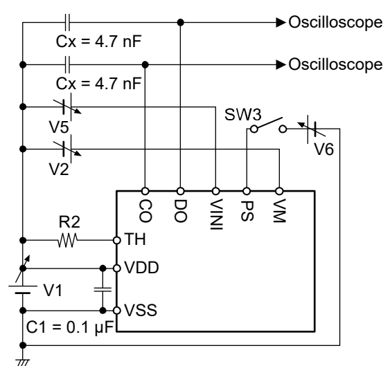
Figure 10 Test Circuit 6
