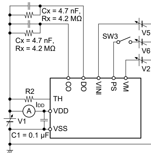
Figure 7 Test Circuit 3
