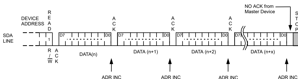
Figure 17 Sequential Read
