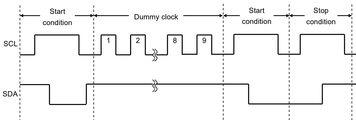
Figure 25 Resetting S-24CS01A/02A/04A
