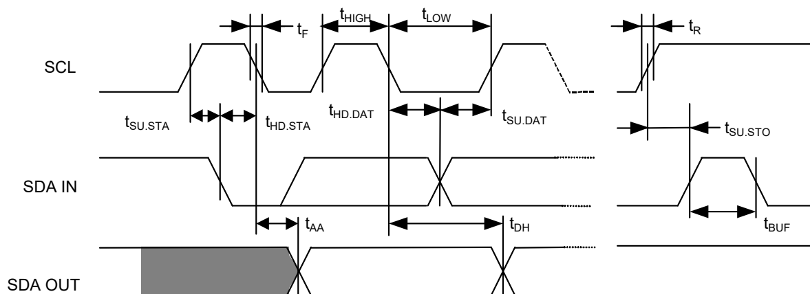
Figure 6 Bus Timing
