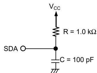
Figure 5 Output Load Circuit
