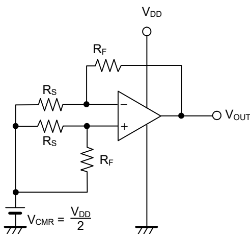
Figure 3 Test Circuit 1
