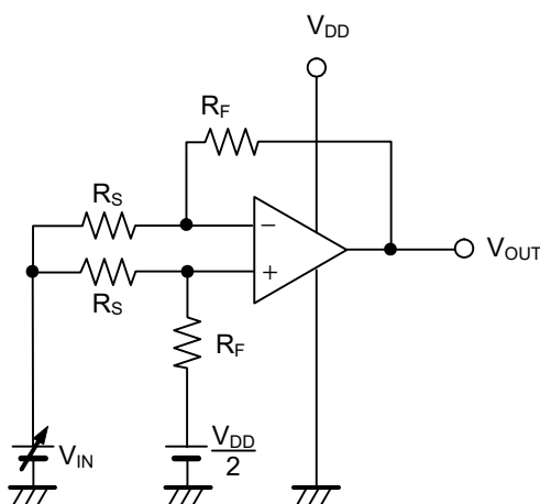
Figure 4 Test Circuit 2
