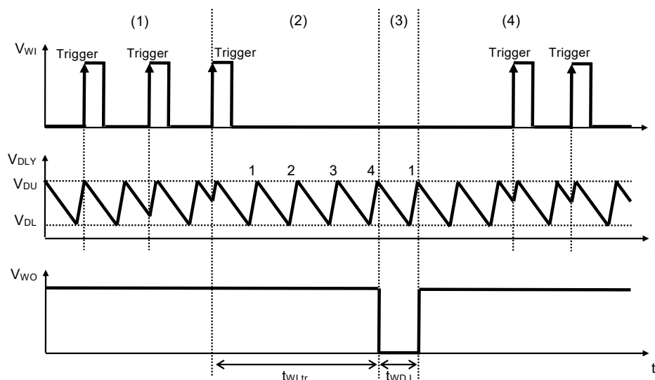
Figure 35 Timing Chart of Watchdog Timer Block
