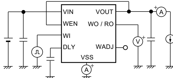
Figure 19 Test Circuit 10
