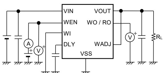
Figure 18 Test Circuit 9
