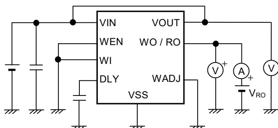
Figure 14 Test Circuit 5
