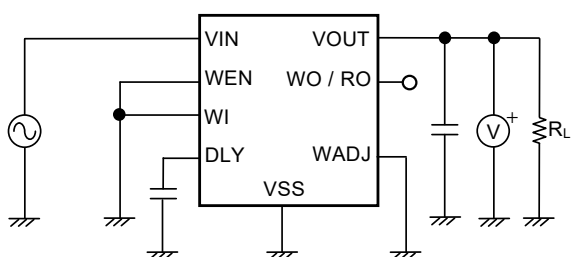
Figure 12 Test Circuit 3
