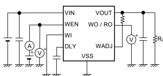
Figure 17 Test Circuit 8
