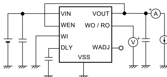
Figure 15 Test Circuit 6
