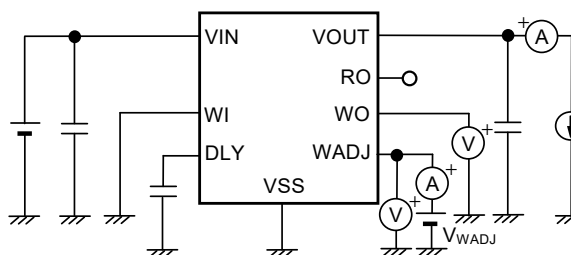
Figure 26 Test Circuit 7
