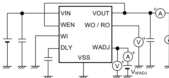
Figure 16 Test Circuit 7
