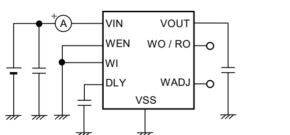
Figure 19 Test Circuit 10
