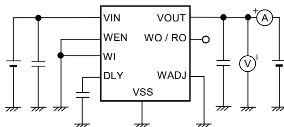
Figure 11 Test Circuit 2
