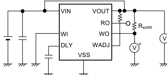
Figure 29 Test Circuit 10
