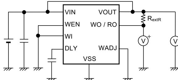
Figure 13 Test Circuit 4
