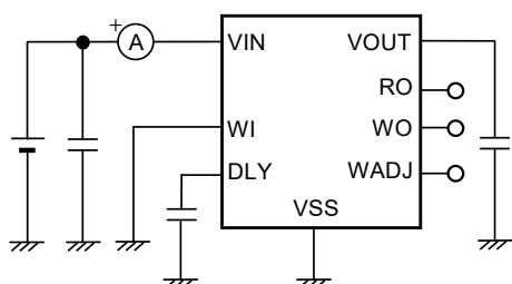
Figure 28 Test Circuit 9
