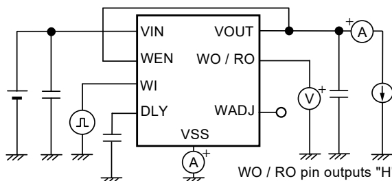
Figure 18 Test Circuit 9
