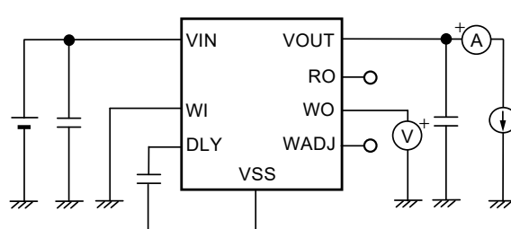
Figure 25 Test Circuit 6
