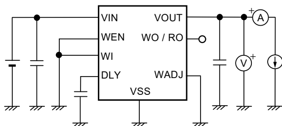
Figure 10 Test Circuit 1
