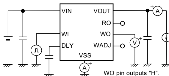
Figure 27 Test Circuit 8
