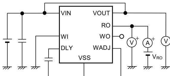
Figure 24 Test Circuit 5
