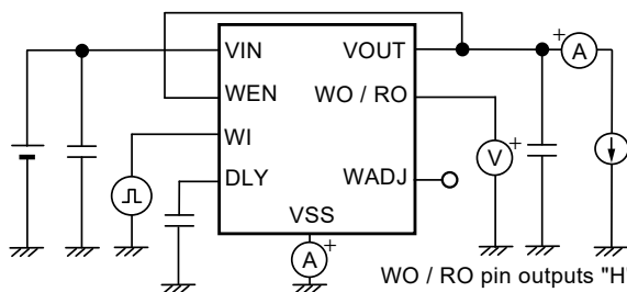
Figure 18 Test Circuit 9
