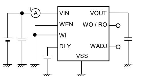
Figure 19 Test Circuit 10
