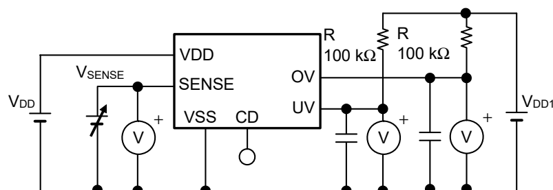
Figure 38 Test Circuit of Response Time
