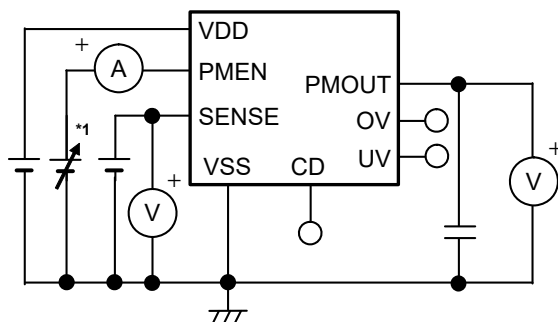
Figure 8 Test Circuit 4
