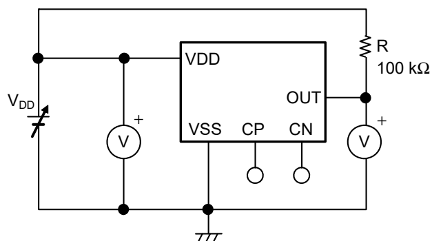
Figure 8 Test Circuit 1 (VDD Detection Product)
