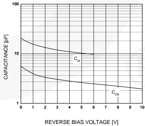
Figure 6. Input and Output Capacitance vs. Reverse Voltage
