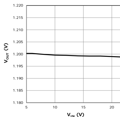
Figure 2: XR76115 line regulation
