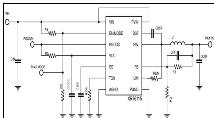
Figure 1: XR76115 Application Diagram
