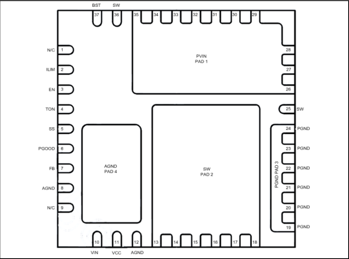
Figure 4: XR76115 Pin Assignment, top view
