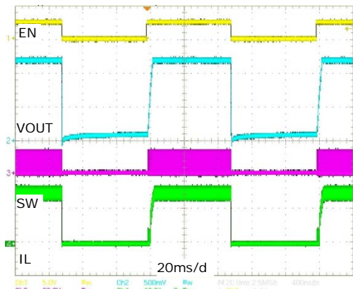
Figure 21: Enable turn on/turn off, 1.2V_{OUT} , 15A
