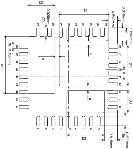
RECOMMENDED PCB LAND PATTERN
