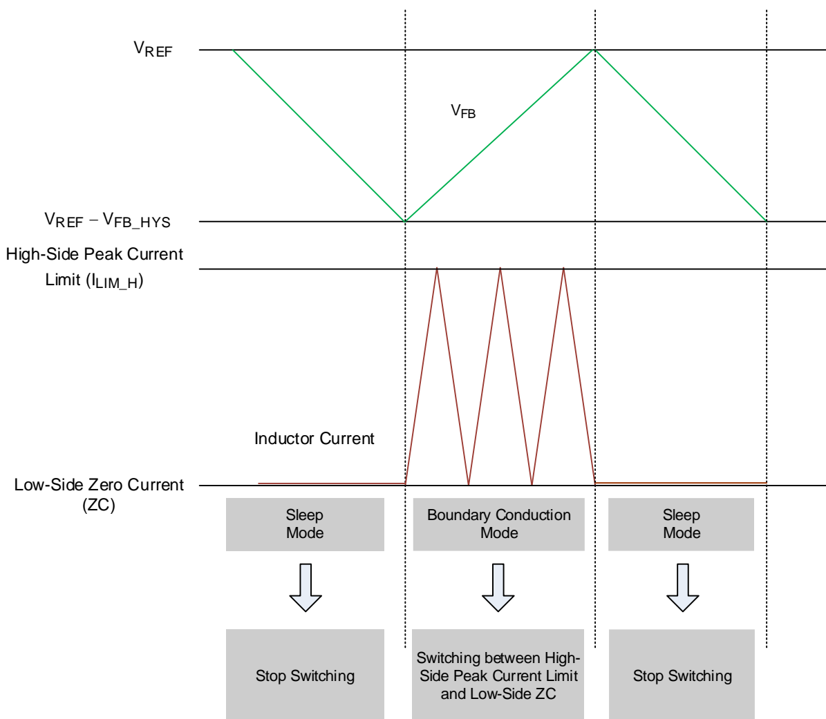
Figure 1. Hysteresis Mode Control
