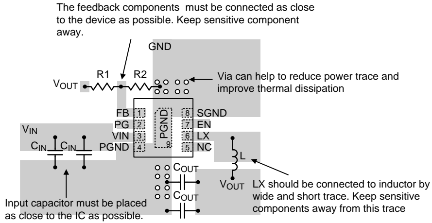
Figure 3. PCB Layout Guide
