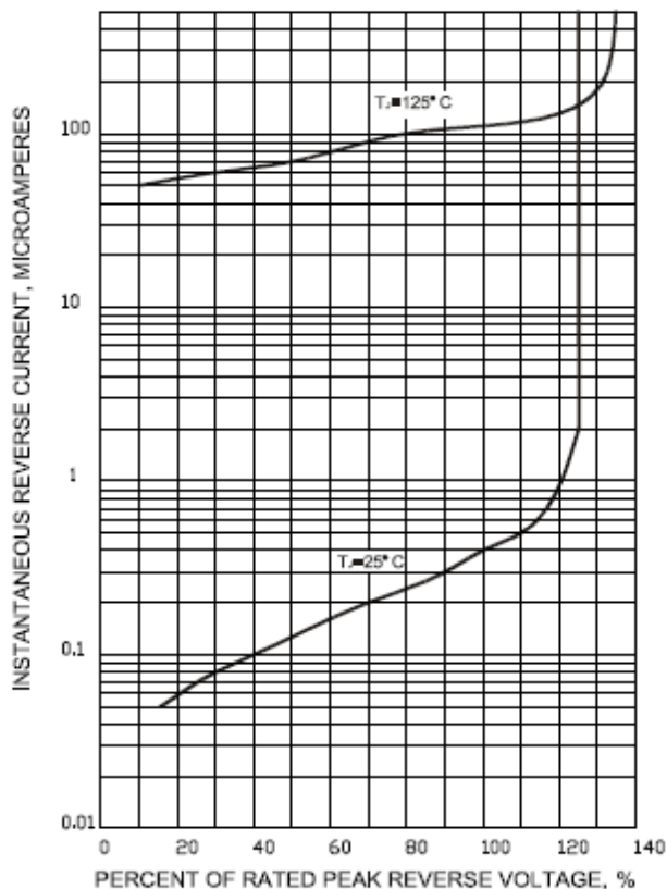
FIG.6-TYPICAL REVERSE CHARACTERISTICS
