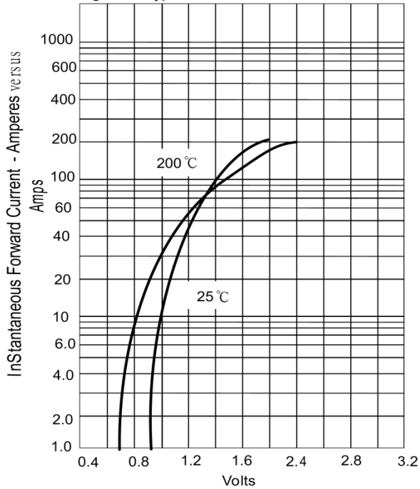
Figure .3-Peak Forward Surge Current
