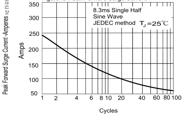
Figure .3-Peak Forward Surge Current
