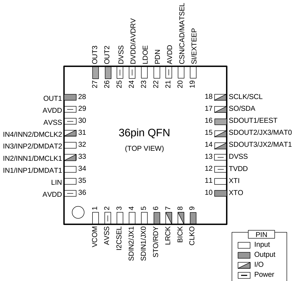
Figure 3. Pin Layout
