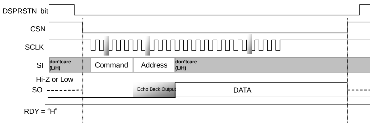
Figure 61. RAM Reading during System Reset/RUN (SPI)
