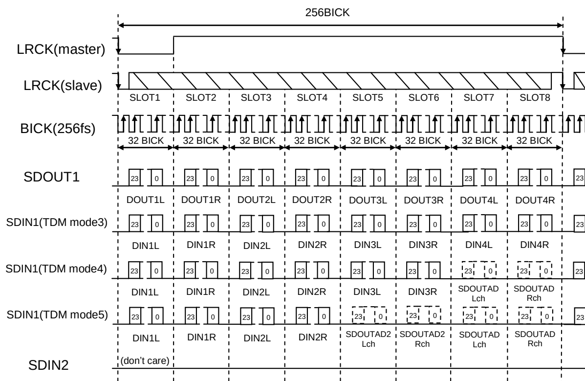
Figure 44. TDM mode I²S Compatible (Internal signals are indicated by dotted lines)
