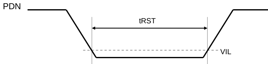
Figure 5. Reset Timing
