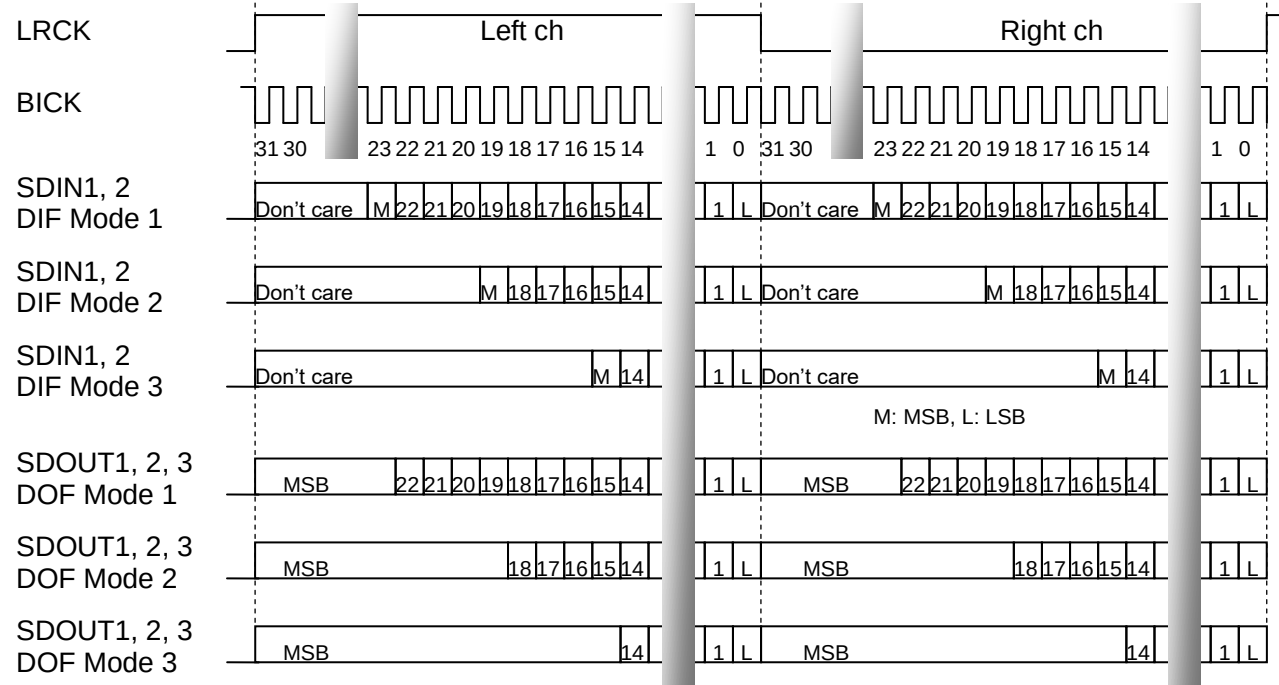
Figure 34. LSB Justified BICK 64fs
