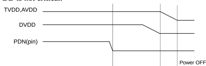
Figure 29. Power-down Sequence
