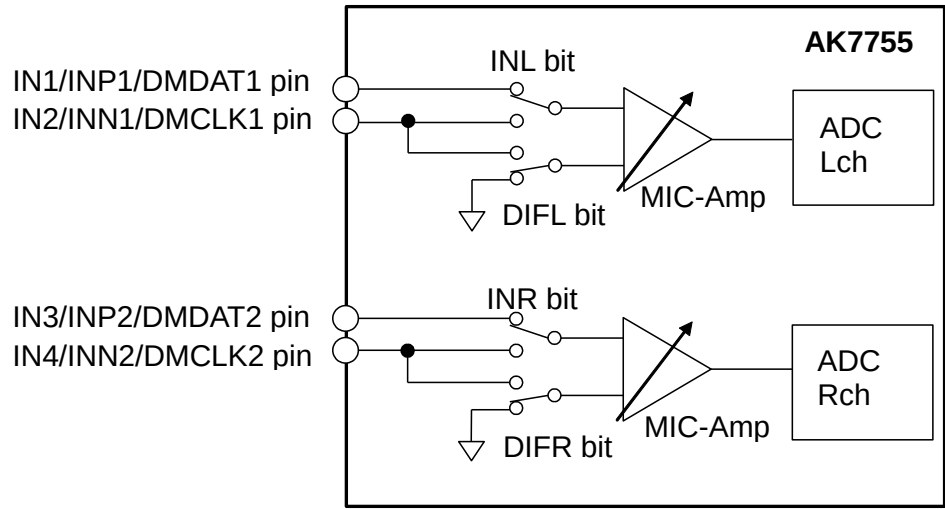
Figure 70. Microphone Input Selector
