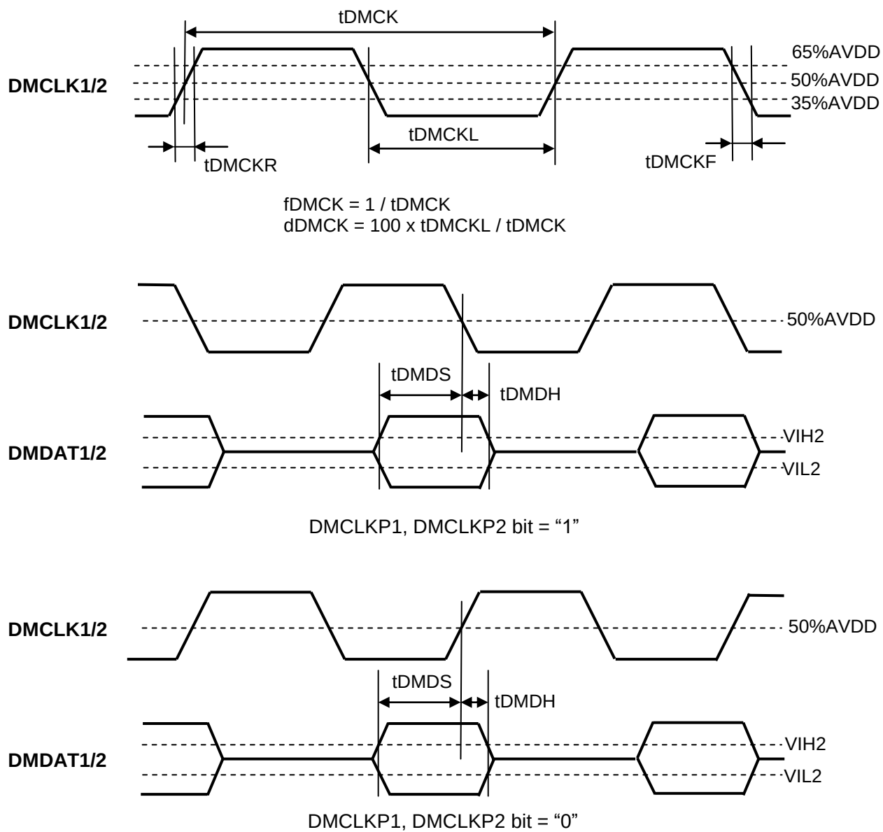
Figure 15. Digital Microphone Interface Timing Wave Form
