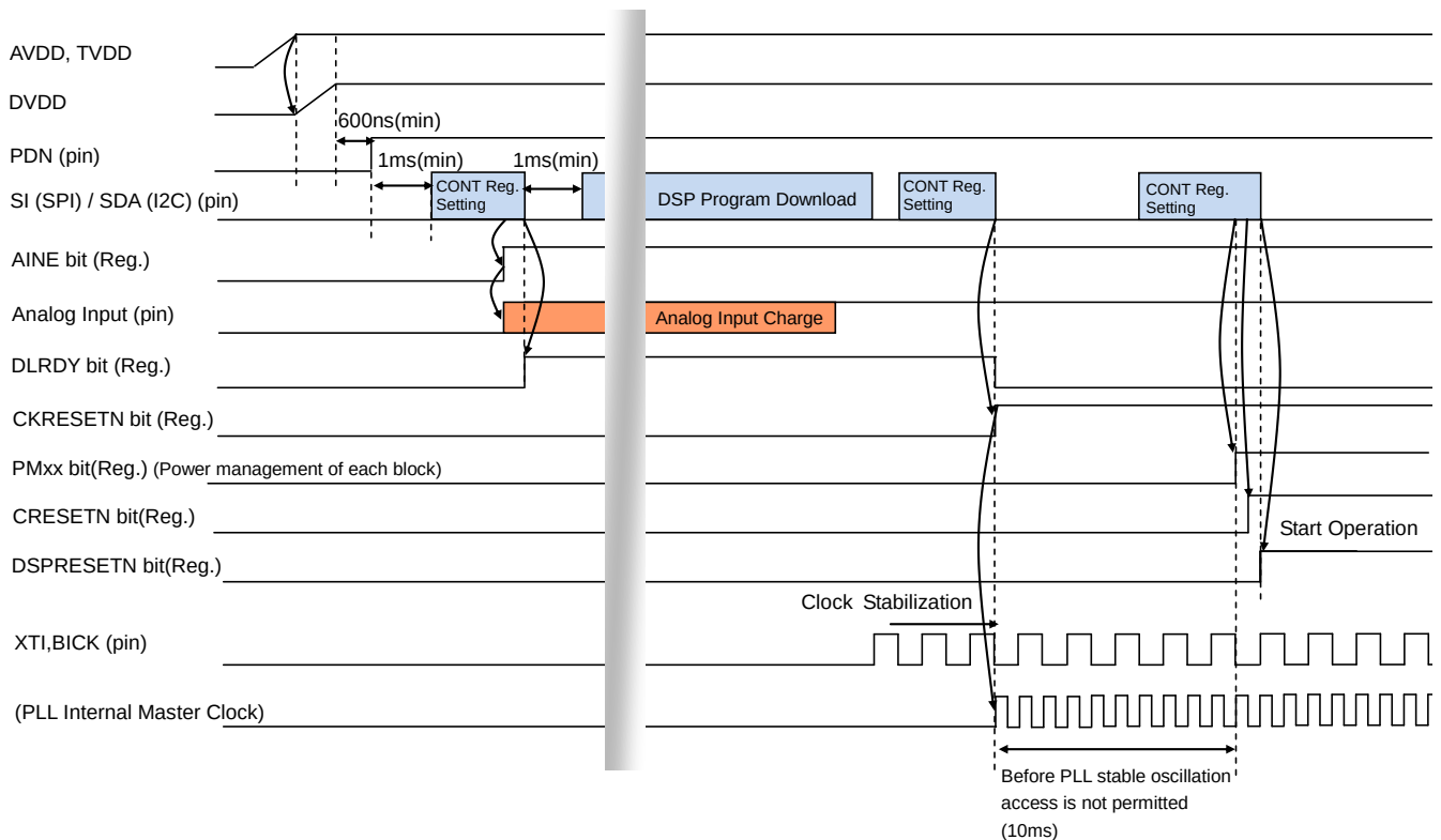
Figure 25. Power-up Sequence 2
