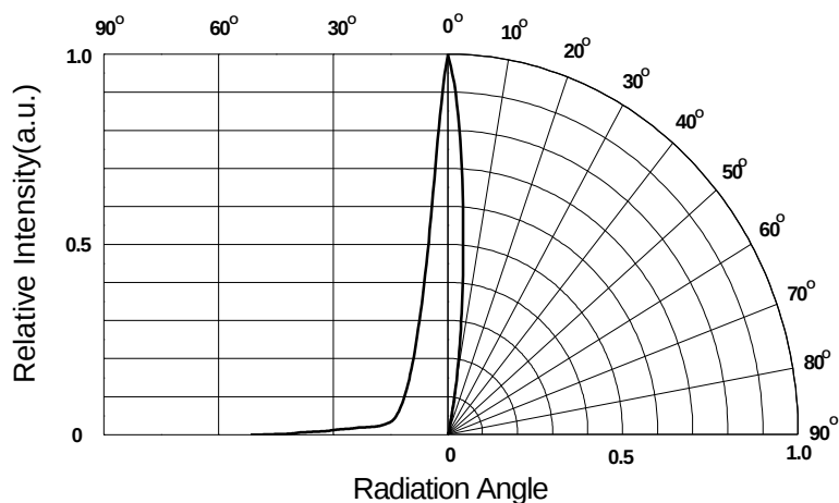
Radiation Characteristics
