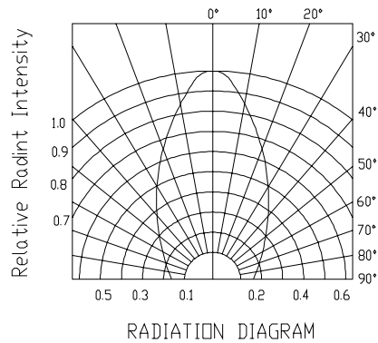
Radiation Diagram T a =25°
