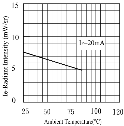
Relative Intensity vs. Ambient Temperature(°C)
