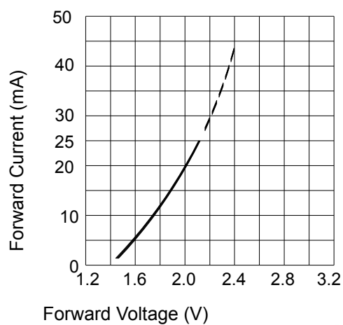
Forward Current vs. Forward Voltage ( T_a=25^\circ )
