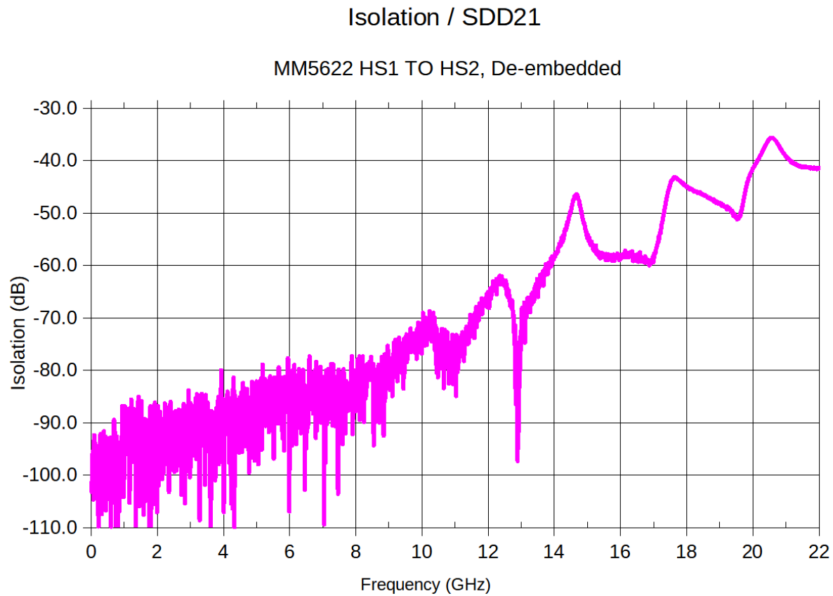
Figure 7. Isolation/SDD21
