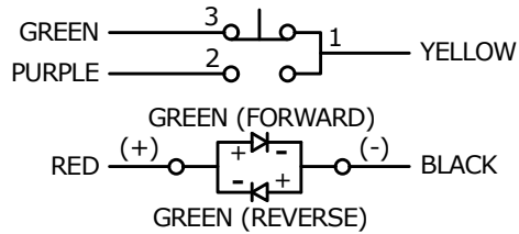
SCHEMATIC SPDT ILLUMINATED FUNCTION ON-ON
