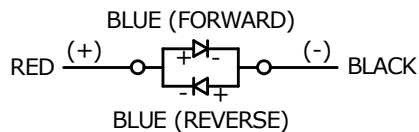
SCHEMATIC
