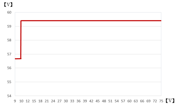
Max adjustable output voltage vs. input voltage at TP_1 = +25 °C. Max adjustable output voltage \geq 56.7 V at V_i = 9 V, P_o = 200 W
