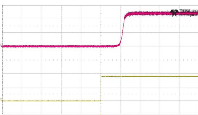
Start-up enabled by connecting V_i at: T_{P1} = +25^{\circ}\text{C} , V_i = 36\text{ V} , I_o = 16.7\text{ A} resistive load. Top trace: output voltage (20 V/div.). Bottom trace: input voltage (5 V/div.). Time scale: (50 ms/div.).
