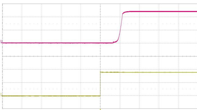
Start-up enabled by connecting V_i at: T_{P1} = +25^\circ\text{C} , V_i = 36\text{ V} , I_o = 4.2\text{ A} resistive load. Top trace: output voltage (20 V/div.), Bottom trace: input voltage (20 V/div.), Time scale: (50 ms/div.).
