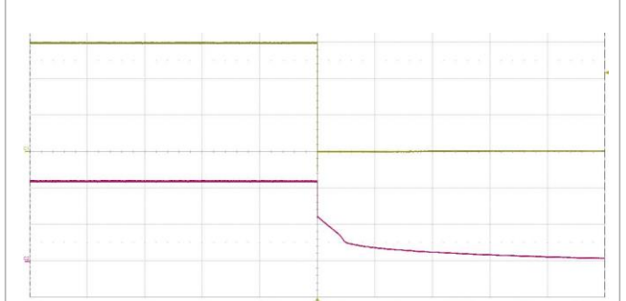
Shut-down enabled by disconnecting V_i at: T_{P1} = +25^{\circ}\text{C} , V_i = 110\text{ V} , I_o = 10\text{ A} resistive load. Top trace: output voltage (5 V/div.). Bottom trace: input voltage (50 V/div.). Time scale: (500 ms/div.).
