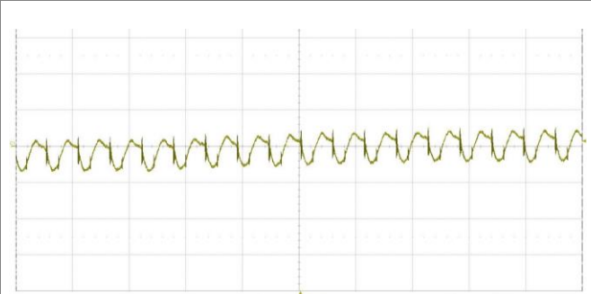
Output voltage ripple at: T_{P1} = +25^\circ\text{C} , V_i = 110\text{ V} , I_o = 4.16\text{ A} resistive load. Trace: output voltage (20 mV/div.). Time scale: (5 \mu\text{s} /div.).
