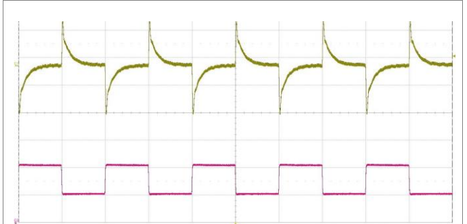
Output voltage response to load current step-change (2.08-3.12-2.08 A) at: T_{P1} = +25^\circ\text{C} , V_i = 110\text{ V} . Trace: output voltage (200 mV/div.). Bottom trace: load current (1 A/div.). Time scale: (1ms/div.).
