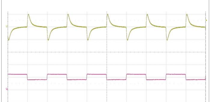
Output voltage response to load current step- change (4.15-6.225-4.15 A) at: T_{P1} = +25^{\circ}\text{C} , V_I = 110\text{ V} . Trace: output voltage (500 mV/div.). Bottom trace: load current (5 A/div.). Time scale: (1ms/div.).
