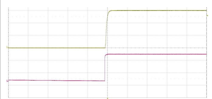
Start-up enabled by connecting V_i at: T_{P1} = +25^\circ\text{C} , V_i = 110\text{ V} , I_o = 6.67\text{ A} resistive load. Top trace: output voltage (5 V/div.). Bottom trace: input voltage (50 V/div.). Time scale: (200 ms/div.).
