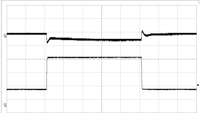
Output voltage response to load current step- change 24-72-24 A (2 A/ \mu\text{s} ) at: T_{PI} = +25^\circ\text{C} , V_I = 53\text{ V} . Top trace: output voltage 500 mV/div. Bottom trace: load current 20 A/div. Time scale: 1 ms/div.
