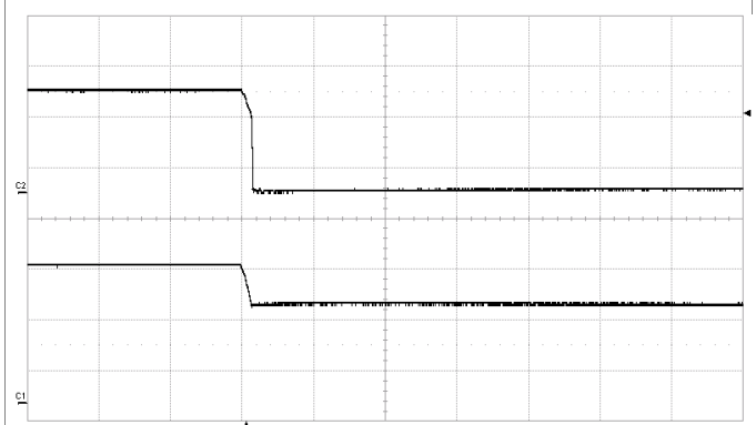
Shut-down enabled by disconnecting V_I at: T_{PI} = +25^\circ\text{C} , V_I = 53\text{ V} , I_O = 96.2\text{ A} resistive load. Top trace: output voltage 5 V/div. Bottom trace: input voltage 20 V/div. Time scale: 2 ms/div.
