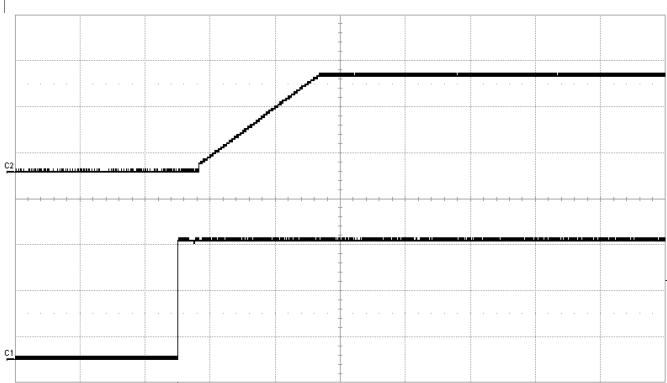
Start-up enabled by connecting V_I at: T_{PI} = +25^\circ\text{C} , V_I = 53\text{ V} , I_O = 96.2\text{ A} resistive load. Top trace: output voltage 5 V/div. Bottom trace: input voltage 20 V/div. Time scale: 100 ms/div.
