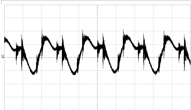
Output voltage ripple at: T_{PI} = +25^\circ\text{C} , V_I = 53\text{ V} , I_O = 96.2\text{ A} resistive load. Trace: output voltage 20 mV/div. Time scale: 2 \mu\text{s} /div.
