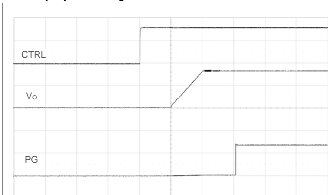
Start-up enabled by CTRL signal. T_{ON\_DELAY} = T_{ON\_RISE} = 10\text{ ms} (default). V_i = 12\text{ V} , I_o = \text{max } I_o , PG pulled up to V_o . Scale: 2 or 1 V/div, 10 ms/div.
