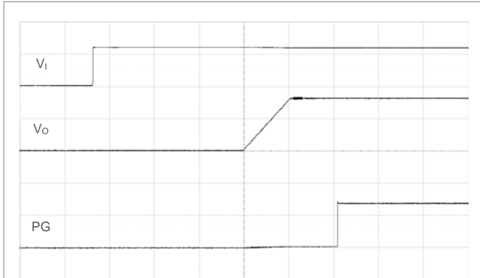
Start-up enabled by applying V_i . T_{ON\_DELAY} = T_{ON\_RISE} = 10\text{ ms} (default). V_i = 12\text{ V} , I_o = \text{max } I_o , PG pulled up to V_o . Scale: 10 or 1 V/div, 10 ms/div.
