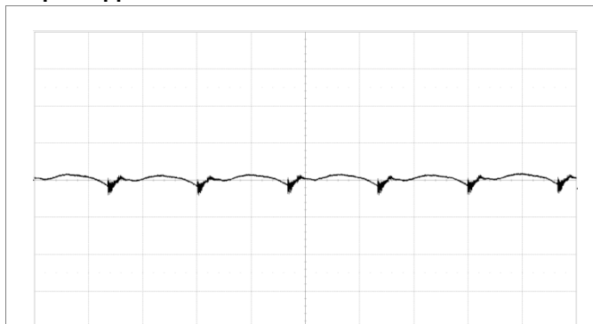
Fundamental output voltage ripple at V_i = 12\text{ V} , C_o = 3 \times 100\ \mu\text{F} , I_o = 12\text{ A} . Scale: 5 mV/div, 1 μs/div, 20 MHz bandwidth. See section Output Ripple and Noise.
