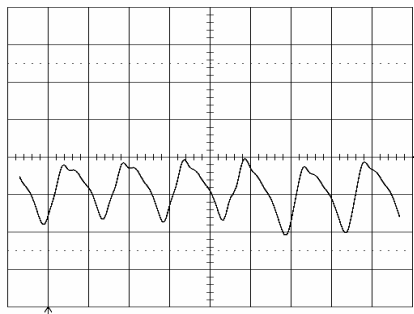
Output voltage ripple (20mV/div.) at: T_{ref} = +25^{\circ}C , I_O = 12 A resistive load, V_i = 12.0 V. Time scale: 2 \mu s/div. See the filter in the Output ripple and noise section (EMC Specification).
