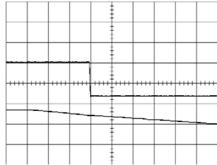
Shut-down enabled by disconnecting V_i at: T_{ref} = +25^{\circ}C , I_O = 12 A resistive load, V_i = 12.0 V. Top trace: output voltage (2.0 V/div.). Bottom trace: input voltage (10 V/div.). Time scale: 5.0 ms/div.
