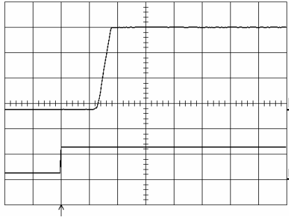
Start-up enabled by connecting V_i at: T_{ref} = +25^{\circ}C , I_O = 12 A resistive load, V_i = 12.0 V. Top trace: output voltage (1.0 V/div.). Bottom trace: input voltage (10 V/div.). Time scale: 10 ms/div.
