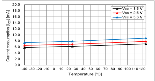
fo = 100 MHz
