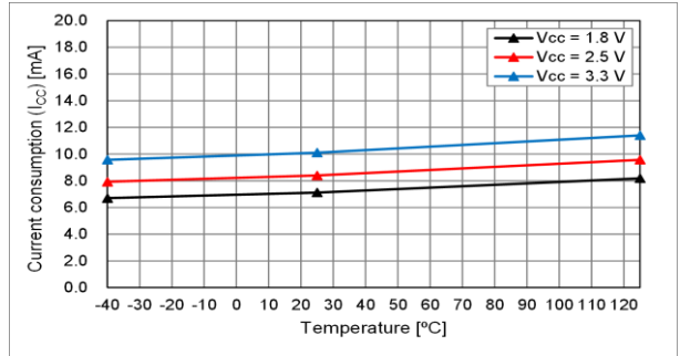
fo = 150 MHz
