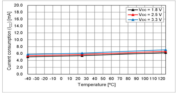
fo = 50 MHz
