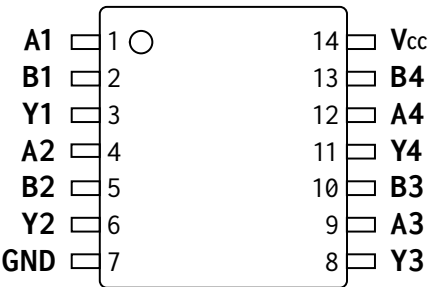
Figure 2: AP54RHC32 device pinout overview
