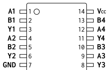
Figure 2: AP54RHC32 device pinout overview
