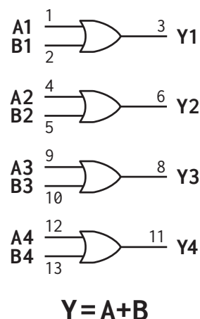
Figure 1: AP54RHC32 logic diagram
