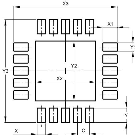
U-QFN4040-20
