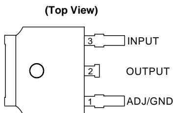
TO252-2 (3) Option 1
