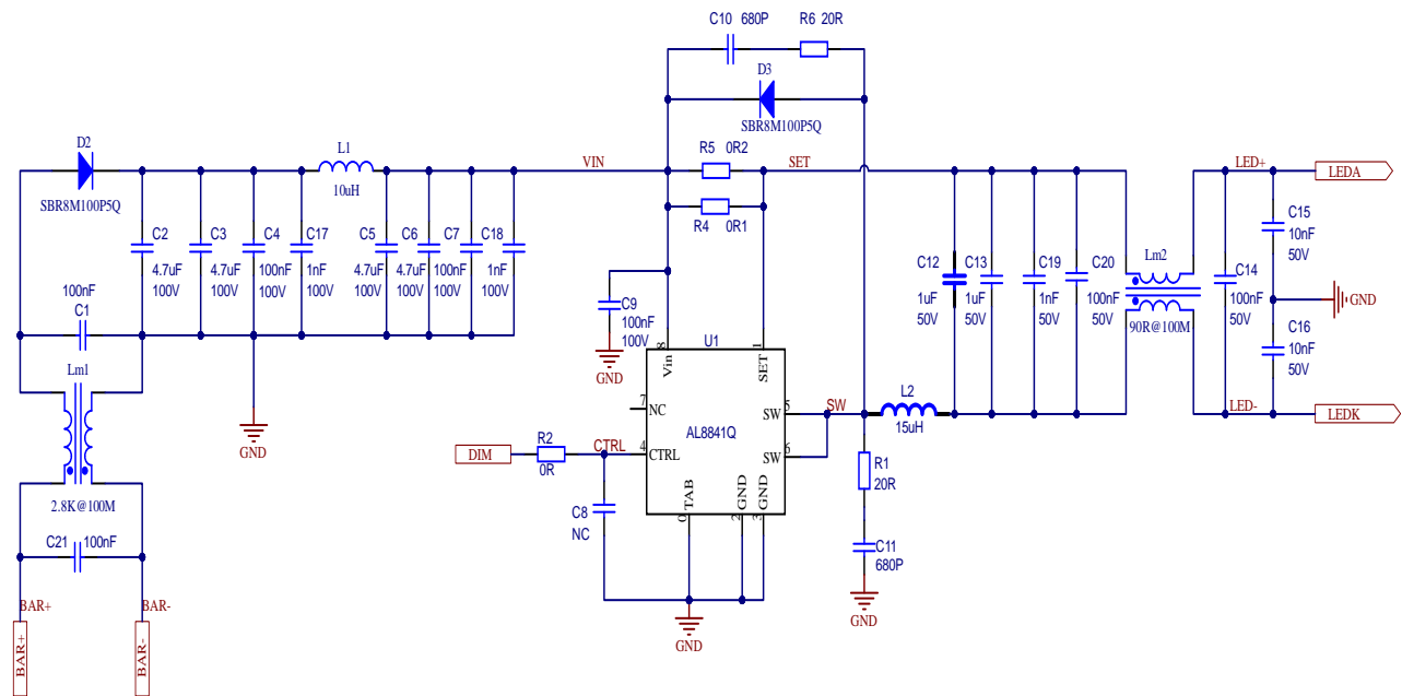
Figure 5: Schematic Circuit
