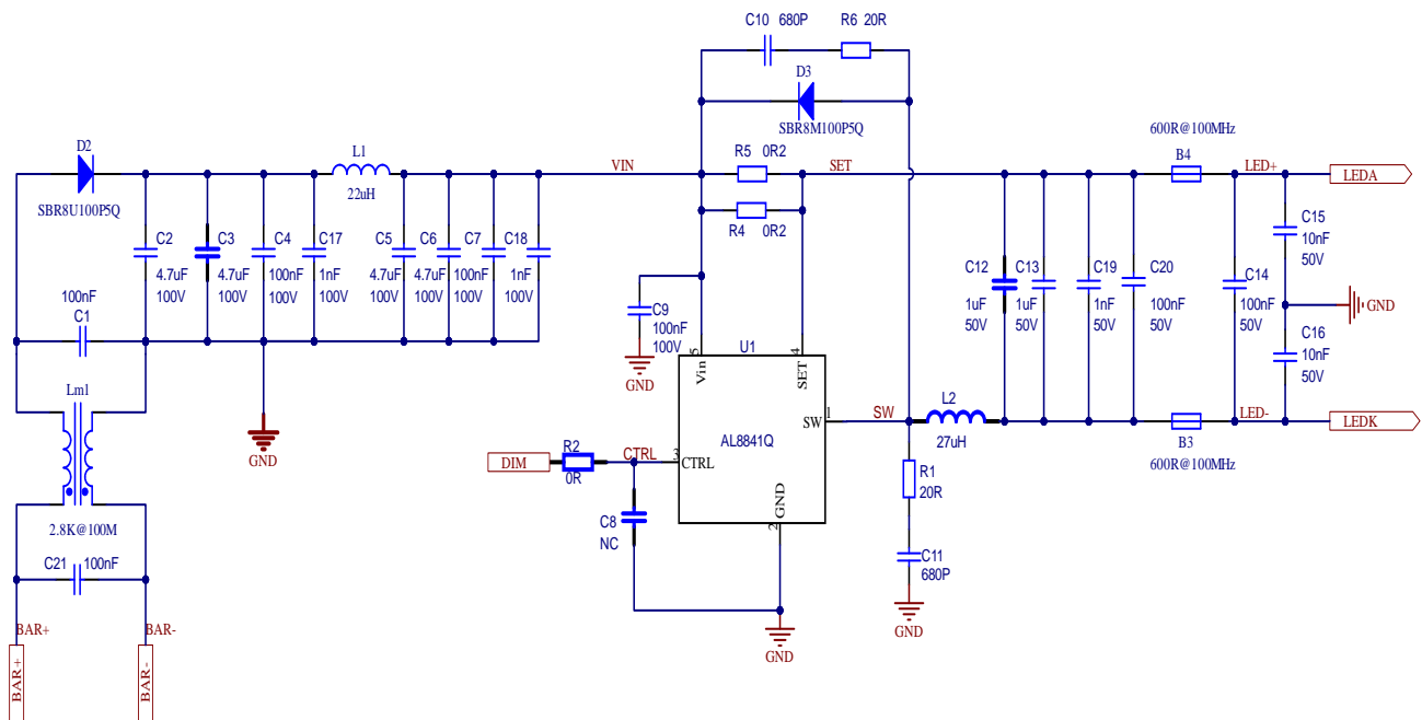
Figure 5: Schematic Circuit
